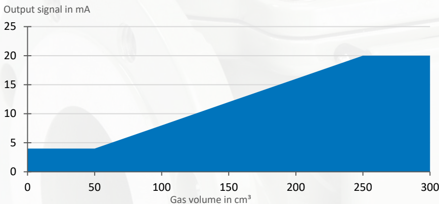
Figure 1 - EXAMPLE COURSE of the output signal with increasing gas volume in the Buchholz relay
